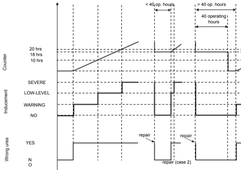
Figure A.8-6. Filling with poor reagent quality
