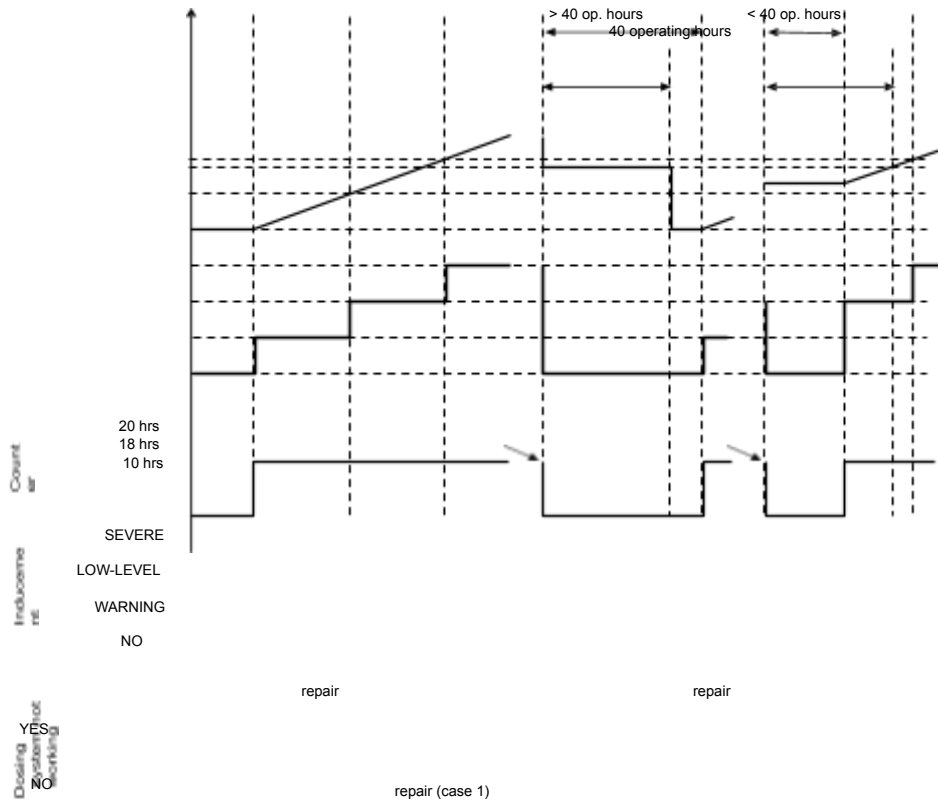
Figure A.8-7. Failure of the reagent dosing system
